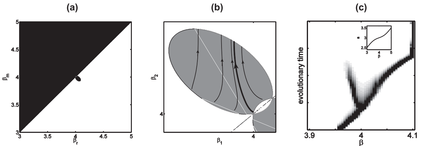
Fig. A1. (a) shows a PIP for the model represented by Eq. (1) with a sinusoidal trade-off in which a(\beta) = 3 + 0.5(\beta - 4) - 0.0145\sin(\pi(\beta - 4)) . Here invadable regions (positive fitness) are black and uninvadable regions (negative fitness) white. (b) shows a TEP with the grey region indicating where two traits can coexist and with representative evolutionary trajectories. (c) shows a simulation of the adaptive dynamics process indicating that traits evolve towards the branching point at \beta = 4 and when nearby undergo disruptive selection to form a dimorphic population. The TEP and the simulations indicate that the dimorphic population will evolve to trait values that cross the boundary of coexistence and here one trait becomes extinct. The trade-off function is shown in the inset figure in (c). Other parameters are b = 1, q = 1, \alpha = 1 and \gamma = 1 .
