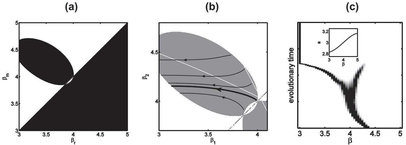
Fig. 5. (a) shows a PIP for the model represented by Eq. (1) with a quartic trade-off in which \alpha = f(\beta) = -0.01\beta^4 + 0.1007651515\beta^3 - 0.2434999998\beta^2 - 0.1014545467\beta + 3.412848488 . Here invadable regions (positive fitness) are black and uninvadable regions (negative fitness) white. (b) shows a TEP with the grey region indicating where two traits can coexist, isoclines represented by white lines and with representative evolutionary trajectories. (c) shows a simulation of the adaptive dynamics process indicating that traits evolve towards the branching point at \beta = 4 and when nearby undergo disruptive selection to form a dimorphic population. The TEP and the simulations indicate that the dimorphic population will evolve to trait values that cross the boundary of coexistence and here one trait becomes extinct. The trade-off function is shown in the inset figure in (c). Other parameters are b = 1, q = 1, \alpha = 1 and \gamma = 1 .
