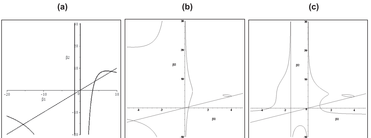
Fig. 4. Extended PIPs showing only zero contours of the fitness and using a broader (often unfeasible) range of \beta . (a) The quadratic example of Fig. 2. (b) The cubic example of Fig. 3. (c) The quartic example of Fig. 5. The diagrams show that in accord with general theory on this broad range, for a trade-off of degree n , there are a maximum of n + 1 singularities and n - 1 simultaneous PIP branches in addition to \beta' = \beta .
