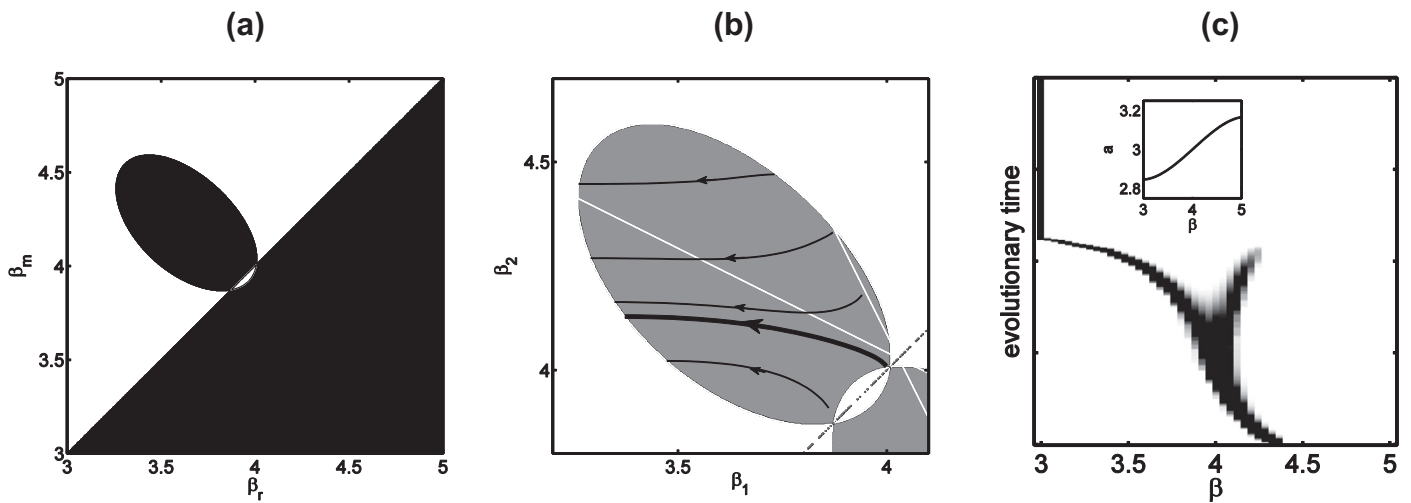
Fig. 3. (a) shows a PIP for the model represented by Eq. (1) with a cubic trade-off in which a = f(\beta) = -0.067234848\beta^3 + 0.8125\beta^2 - 3.045454546\beta + 6.484848483 . Here invadable regions (positive fitness) are black and uninvadable regions (negative fitness) white. (b) shows a TEP with the grey region indicating where two traits can coexist, isoclines represented by white lines and with representative evolutionary trajectories. (c) shows a simulation of the adaptive dynamics process indicating that traits evolve towards the branching point at \beta = 4 and when nearby undergo disruptive selection to form a dimorphic population. The TEP and the simulations indicate that the dimorphic population will evolve to trait values that cross the boundary of coexistence and here one trait becomes extinct. The trade-off function is shown in the inset figure in (c). Other parameters are b = 1, q = 1, \alpha = 1 and \gamma = 1 .
