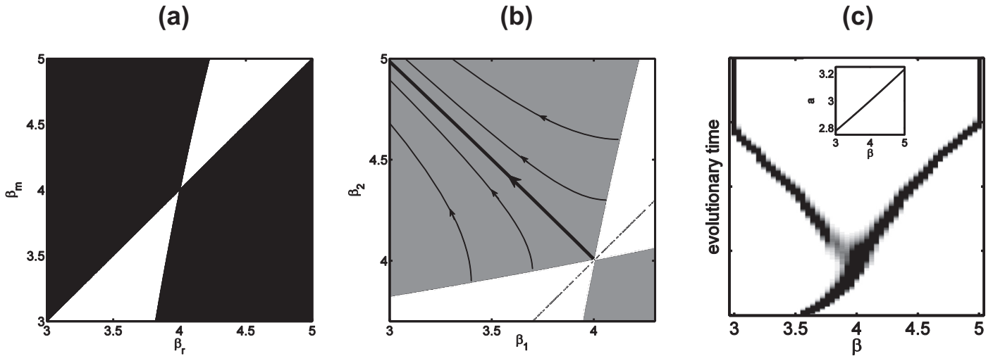
Fig. 2. (a) shows a PIP for the model represented by Eq. (1) with a quadratic trade-off in which a = f(\beta) = 0.0057\beta^2 + 0.1818\beta + 2.1818 . Here invadable regions (positive fitness) are black and uninvadable regions (negative fitness) white. (b) shows a TEP with the grey region indicating where two traits can coexist and with representative evolutionary trajectories. (c) shows a simulation of the adaptive dynamics process indicating that traits evolve towards the branching point at \beta = 4 and when nearby undergo disruptive selection to form a dimorphic population. The TEP and the simulations indicate that the dimorphic population will evolve to be composed of the minimum and maximum trait values. The trade-off function is shown in the inset figure in (c). Other parameters are b = 1, q = 1, \alpha = 1 and \gamma = 1 .
