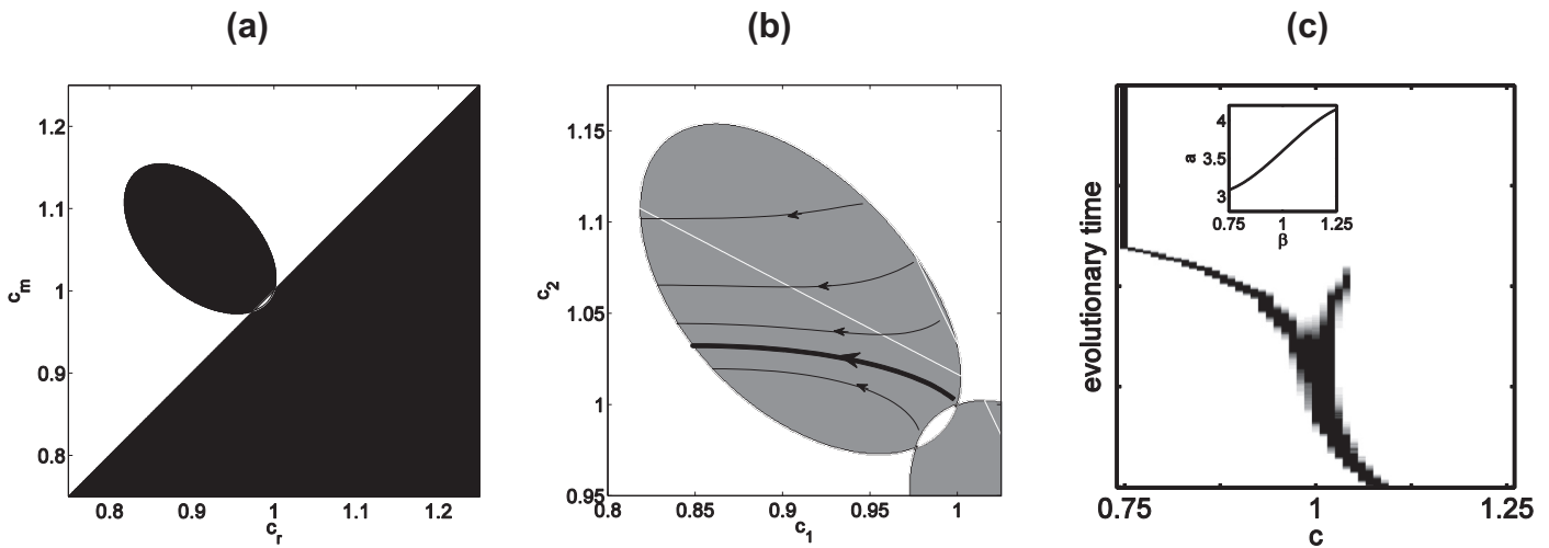
Fig. A2. (a) shows a PIP for the predator-prey model represented by Eq. (B1) with a cubic trade-off in which r(c) = -7.5c^3 + 22.75c^2 - 20.4c + 8.75 . Here invadable regions (positive fitness) are black and uninvadable regions (negative fitness) white. (b) shows a TEP with the grey region indicating where two traits can coexist and with representative evolutionary trajectories. (c) shows a simulation of the adaptive dynamics process indicating that traits evolve towards the branching point at c = 1 and when nearby undergo disruptive selection to form a dimorphic population. The TEP and the simulations indicate that the dimorphic population will evolve to cross the boundary of coexistence and here one trait becomes extinct. The trade-off function is shown in the inset figure in (c). Other parameters are d = 1, e = 1 and h = 1 .
