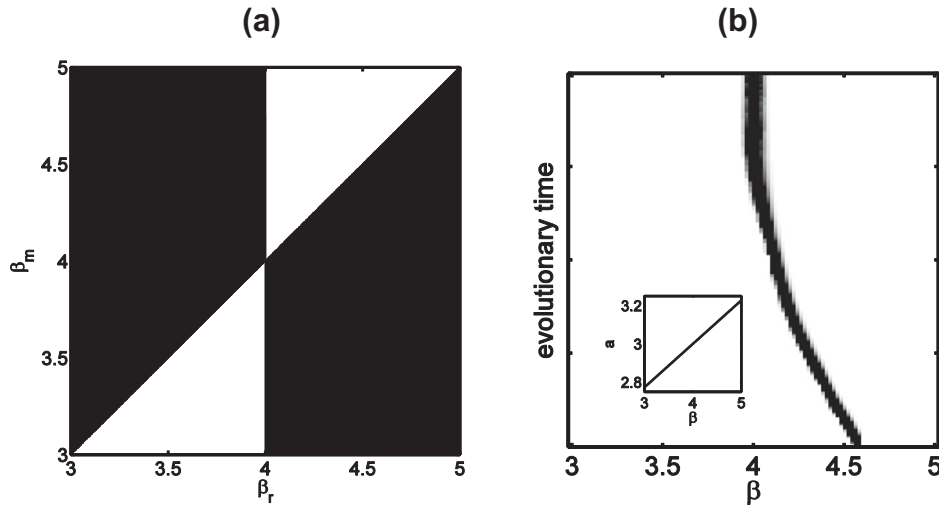
Fig. 1. (a) shows a PIP for the model represented by Eq. (1) with a linear trade-off in which a = f(\beta) = 0.2273\beta + 2.09091 . Here invadable regions (positive fitness) are black and uninvadable regions (negative fitness) white. (b) shows a simulation of the adaptive dynamics process indicating that traits evolve towards the singular point at \beta = 4 . The trade-off function is shown in the inset figure in (b). Other parameters are b = 1 , q = 1 , \alpha = 1 and \gamma = 1 .
