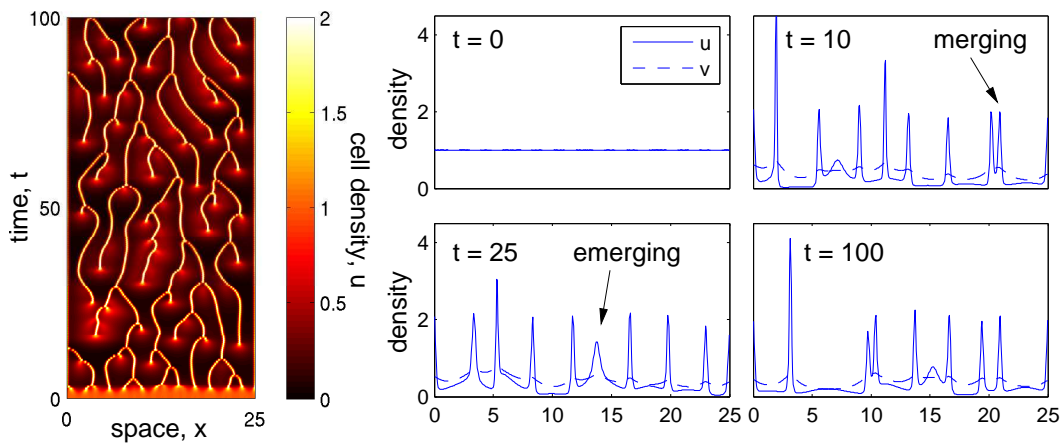
Figure 1: An example of spatio-temporal patterning observed in equations (3)–(4). Left: cell-density ( u ) plotted as a function of space (horizontal axis) and time (vertical axis). The colorscale bar indicates increasing cell density from u = 0 (black) to u \geq 2 (white). The uniform solution destabilises into a number of cellular aggregations which subsequently evolve through an apparently arrhythmic sequence of emerging and merging events. Right: 4 frames showing snapshots of the cell (solid line) and chemical (dashed line) distributions at the times indicated. Examples of merging and emerging events are indicated. For this set of simulations, equations (3)–(4) are solved with D = 0.1 , r = 1.0 , \chi = 5.0 and L = 25 with initial conditions (5) and zero-flux boundary conditions. The numerical method is as described in Section 1.4, here we set \Delta x = L/500 .
